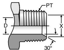
Male Pipe End
